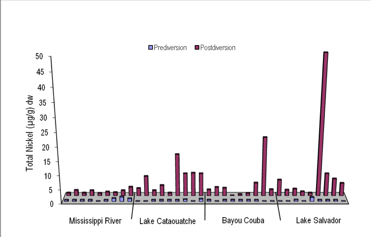
Figure 22B. Three-dimensional comparison of Davis Pond prediversion and postdiversion values for nickel by dry weight (in micrograms per gram [ \mu\text{g/g} ]).
